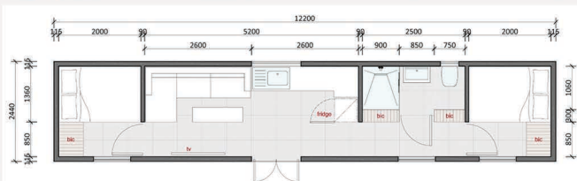
FLOOR PLAN
