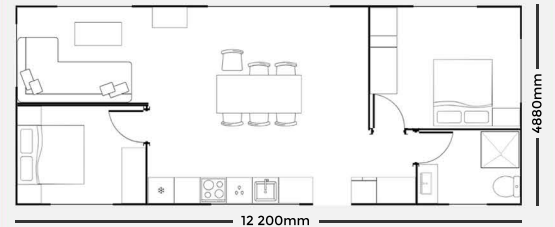
FLOOR PLAN
